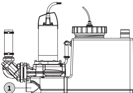
Fig. 7: Connection of diaphragm hand pump
