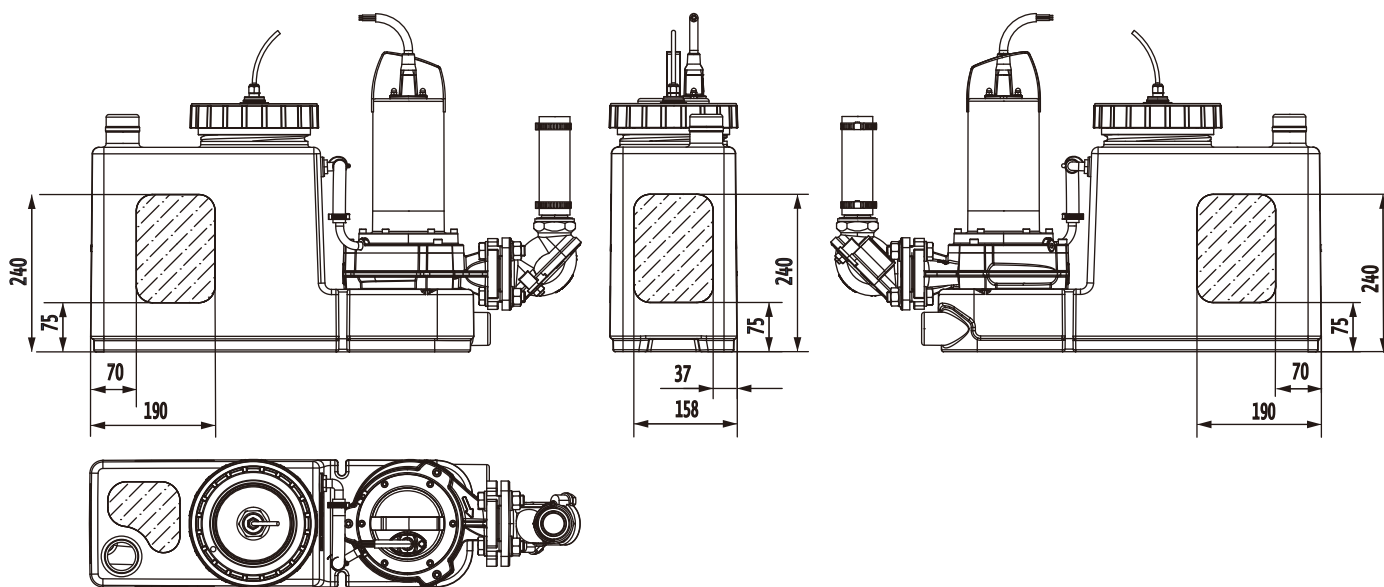
Fig. 4: Inlet areas
