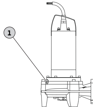
Fig. 6: Sealing chamber oil change
