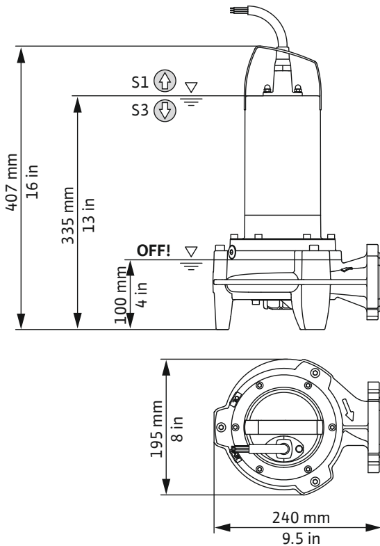
Fig. 3: Installation dimensions
