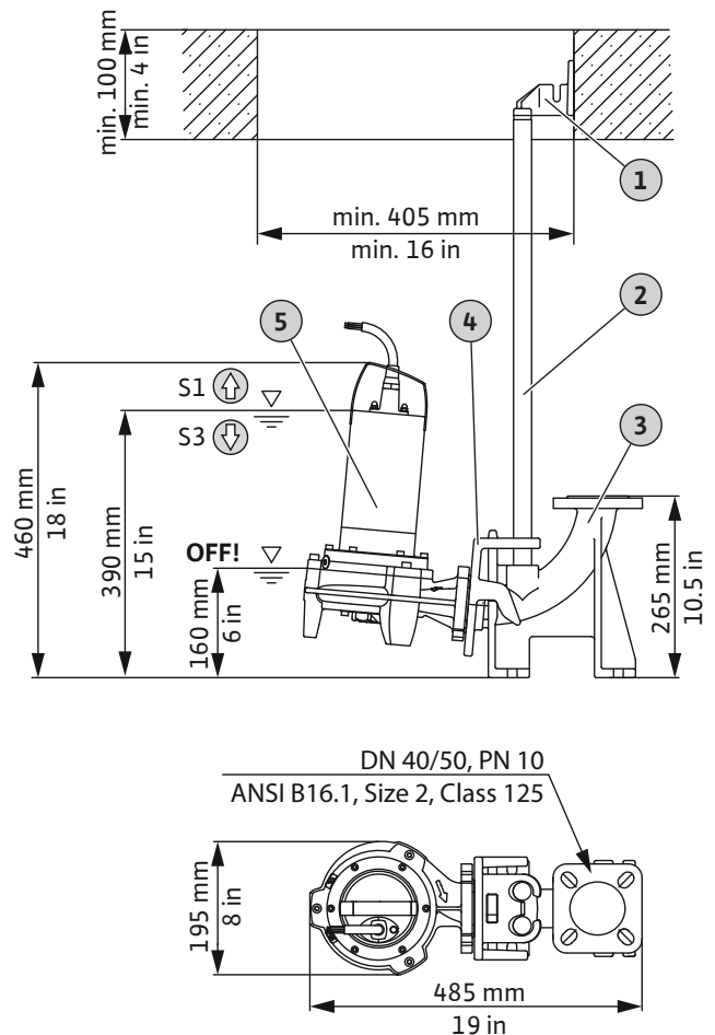
Fig. 2: Overview of components and installation dimensions
